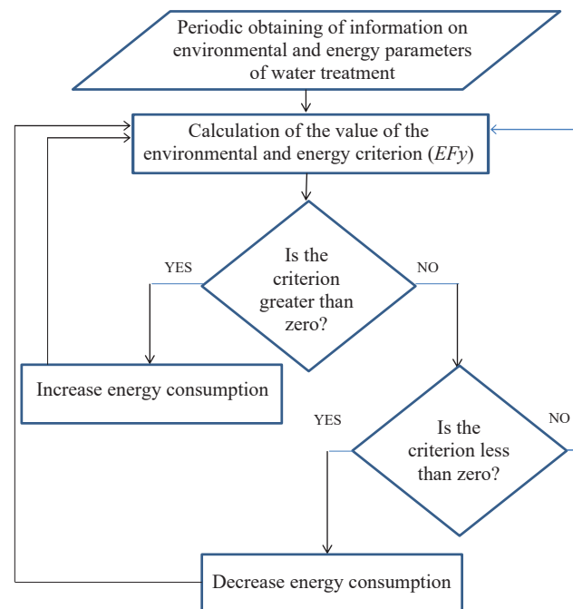
Fig. 1. The block diagram of the algorithm for the practical use of environmental and energy criteria for the treatment of industrial wastewater
