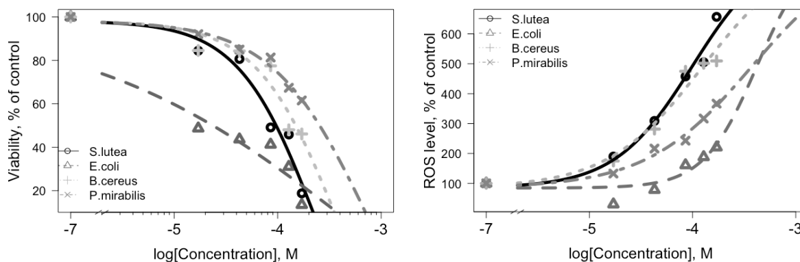
Figure 2. Effect of different concentrations of 2-F-araA with equimolar antioxidant concentrations against exponential phase E. coli , S. lutea , B. cereus , and P. mirabilis (incubated aerobically) at 37 °C for 24 h
