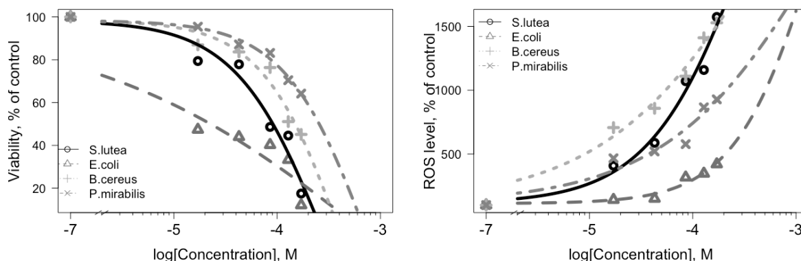
Figure 1. Effect of different concentrations of 2-F-araA without antioxidant against exponential phase E. coli , S. lutea , B. cereus , and P. mirabilis (incubated aerobically) at 37 °C for 24 h
